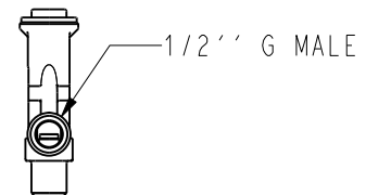
DETAIL SOUPAPE ⑤ & ⑨
