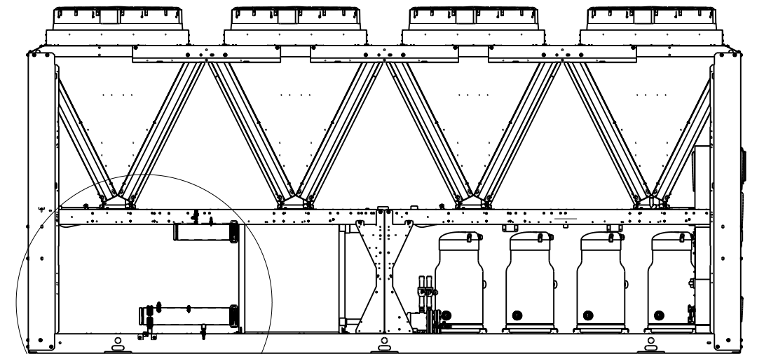
DETAIL SOUPAPE ⑤ & ⑨
