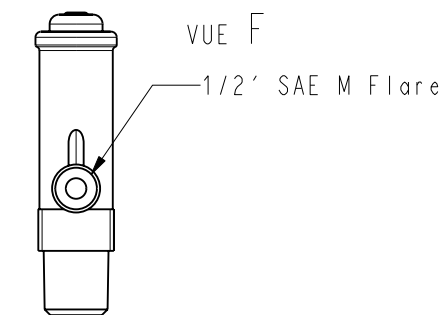
DETAIL SOUPAPE 9
