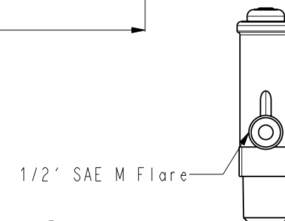
DETAIL SOUPAPE 9
