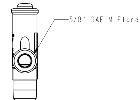
DETAIL SOUPAPE 5
