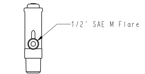
DETAIL SOUPAPE 9
