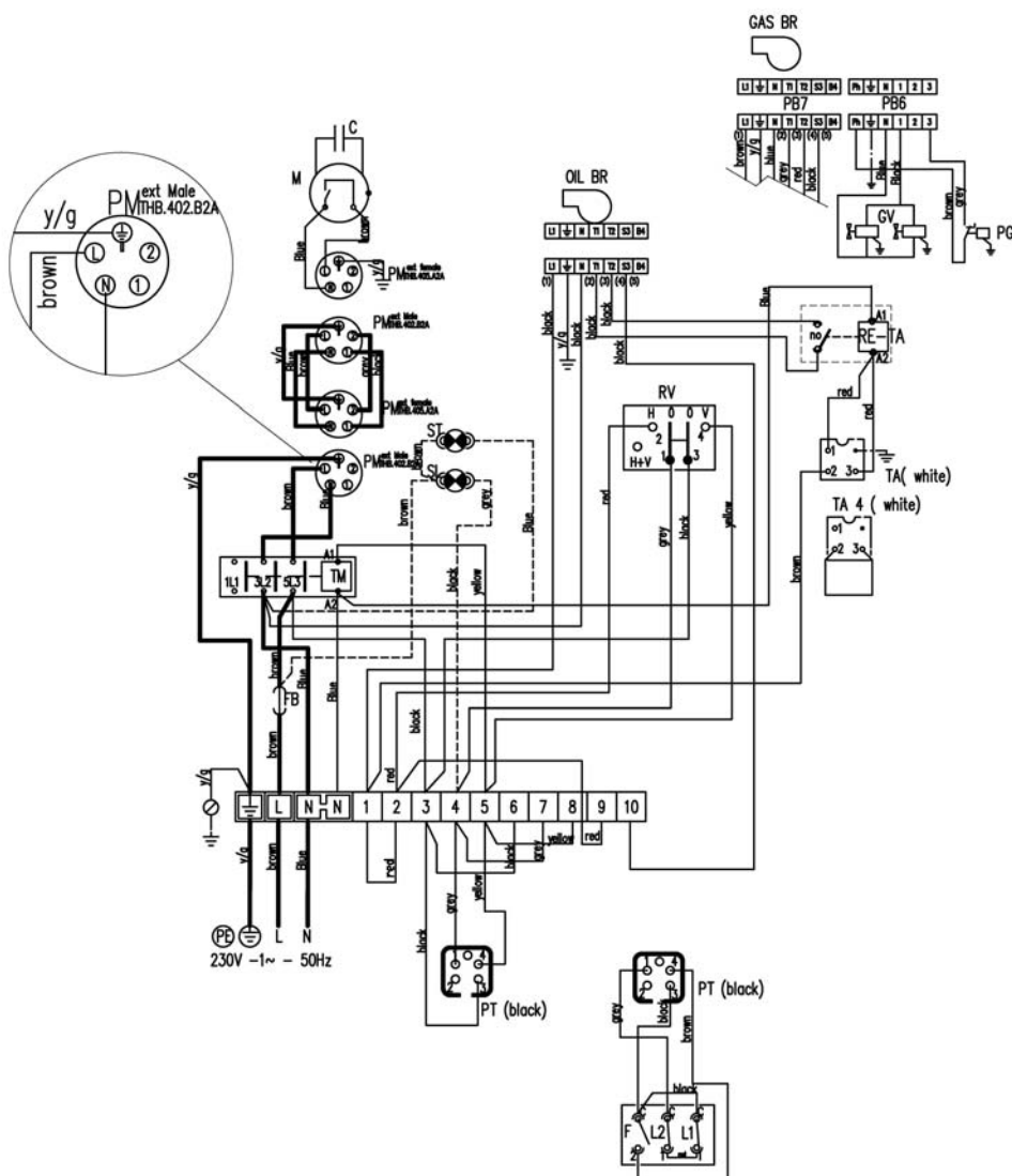
Electronic thermostat : OPTIONAL
