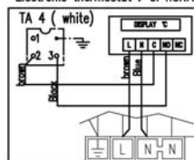
Electronic thermostat : OPTIONAL
