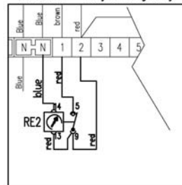
OPTIONAL – delay starting relay
